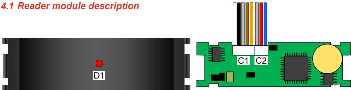
Pic. 2: MREM 80 AgorGR reader module, front (left) and rear (right) view
