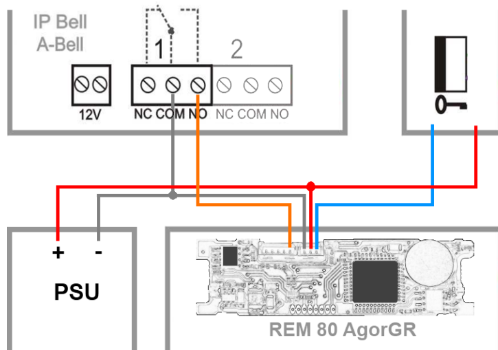
Pic. 3: Standard reader module connection with use DC power supply and the relay contact of the A-Bell / IP Bell entry panel
